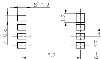
REFERRED FOOTPRINT LAYOUT
